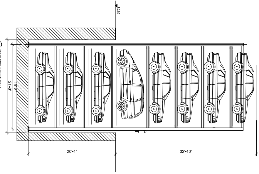
○ LIFT SLIDING SYSTEMS/30B SECTIONAL ELEVATION B/B
